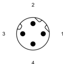
Technical Data Side 1 M12 Male
